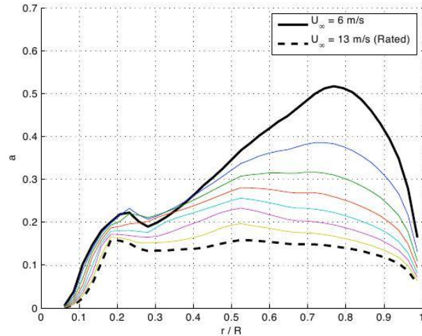
Figure 5: Rotor axial induction factor as a function of the normalized radial position over a range of wind speeds for a constant-speed wind turbine.
