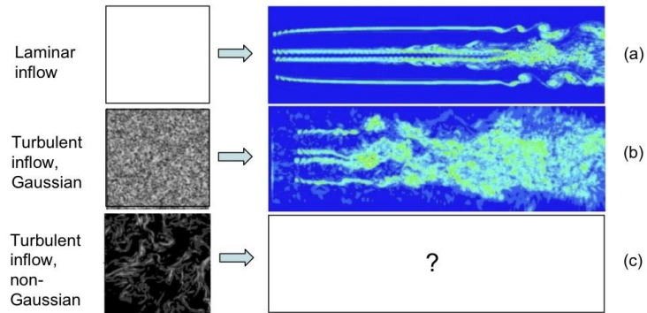
Figure 3: Simulations of wind turbine wakes for varying inflow conditions. (Troldborg et al 2007) (a) laminar inflow and (b) Gaussian synthetic turbulence inflow. Possible effects of non-Gaussian inlet conditions (c) are still an open question (Rosales & Meneveau 2006).
